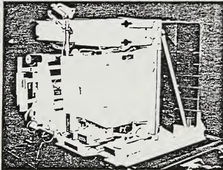
Figure 12 ALSEP Subpackage 2 Heat-Flow-Instrument Subpallet
